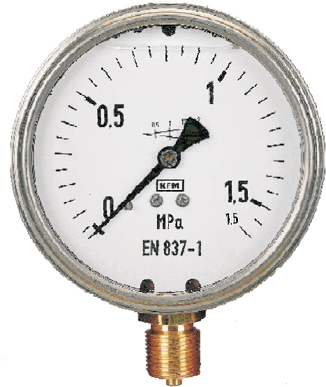
Manometr model 113.53
